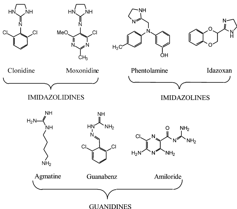
Figure 1. Different families of compounds that interact with the imidazoline binding sites.
