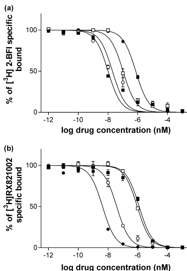
Figure 3. Inhibition of specific binding of [^3H]2 -BFI (A) or [^3H]RX821002 (B) to human brain cortex membranes by Idazoxan ( \circ ), 13 ( \bullet ), 8 ( \square ) and 4 ( \blacksquare ). Each point is the mean \pm SEM of four independent experiments.
