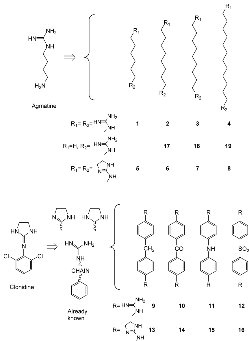
Figure 2. ‘Aliphatic’ compounds (structurally related to agmatine) and ‘aromatic’ compounds (clonidine related structures) proposed and studied as I 2 imidazoline binding sites ligands.
